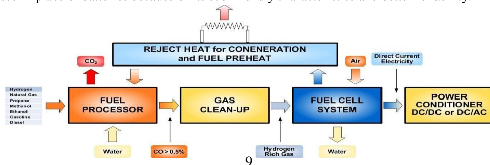
Figure 2. Cogeneration system in fuel cell [6]
