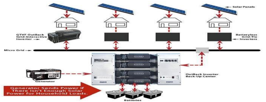
Figure 1: Microgrid system with PV and storage [1]
