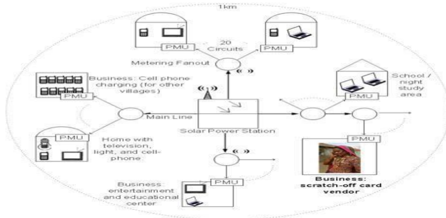
Figure 5. Gram Power Company Microgrid Model in Rajasthan
